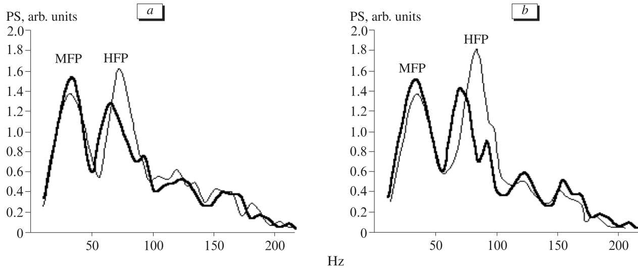
Fig. 2. Effect of electrical stimulation of retrotrapezoid nucleus on power spectrum of phrenic nerve discharges. a ) power spectrum of the first half of respiratory burst before (solid line) and during (thin line) stimulation of the nucleus; b ) corresponding plots for the second half of respiratory burst.
